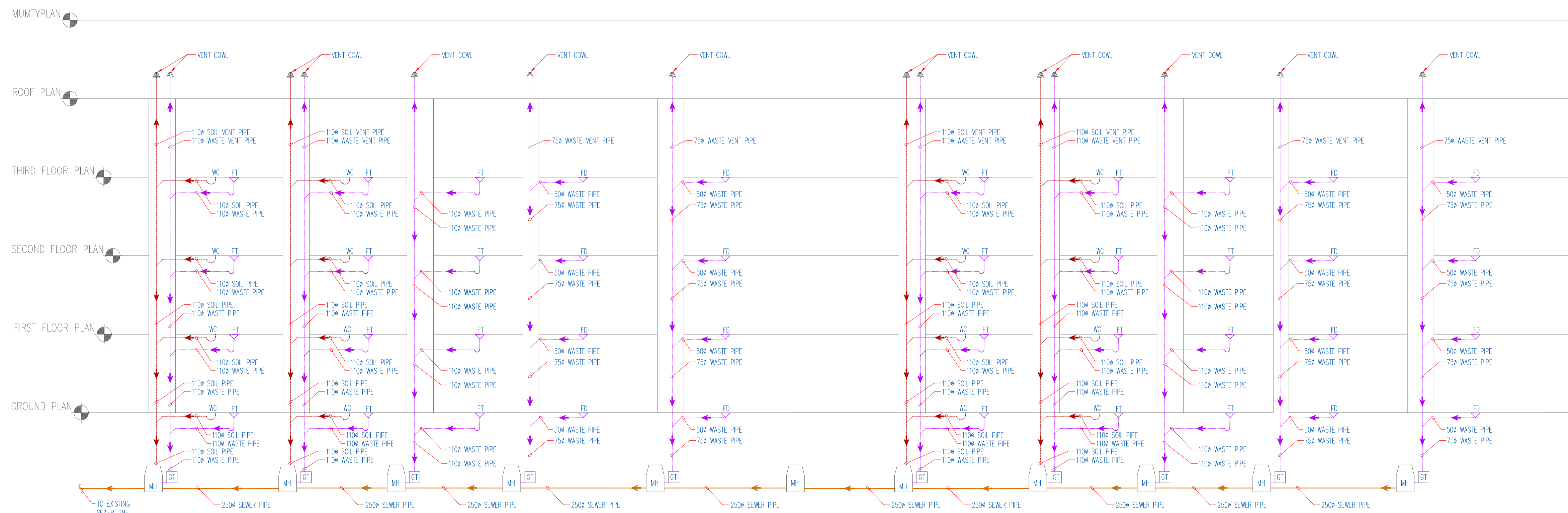
Single Line Diagram : Drainage Layout
